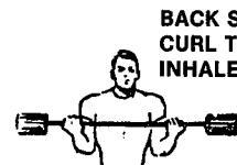
CURL
